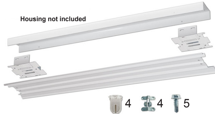
shown above: Reflector 1 Brackets 2 4' Components
