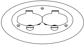
FPT-CACP FPT-CACP-AL Metallic Covers 5¾" Dia.
