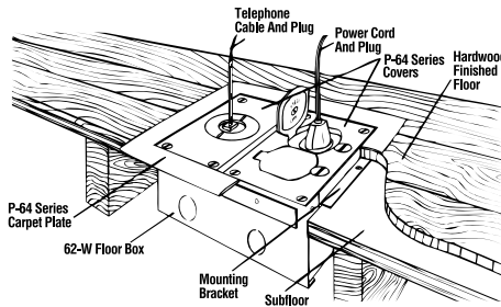
Stamped Steel Floor Box Line for Use in Wood Floors
