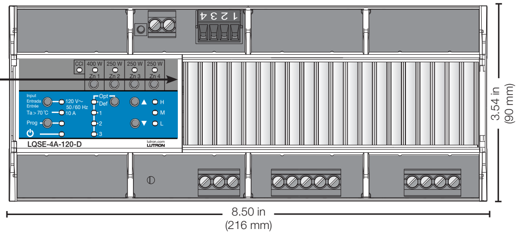
Front View
